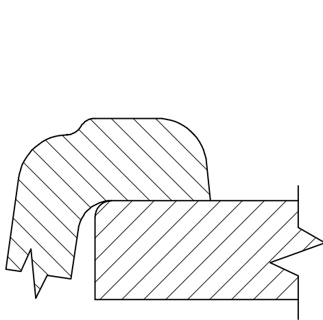
DETAIL SHOWING A DROP-IN INSTALLATION
