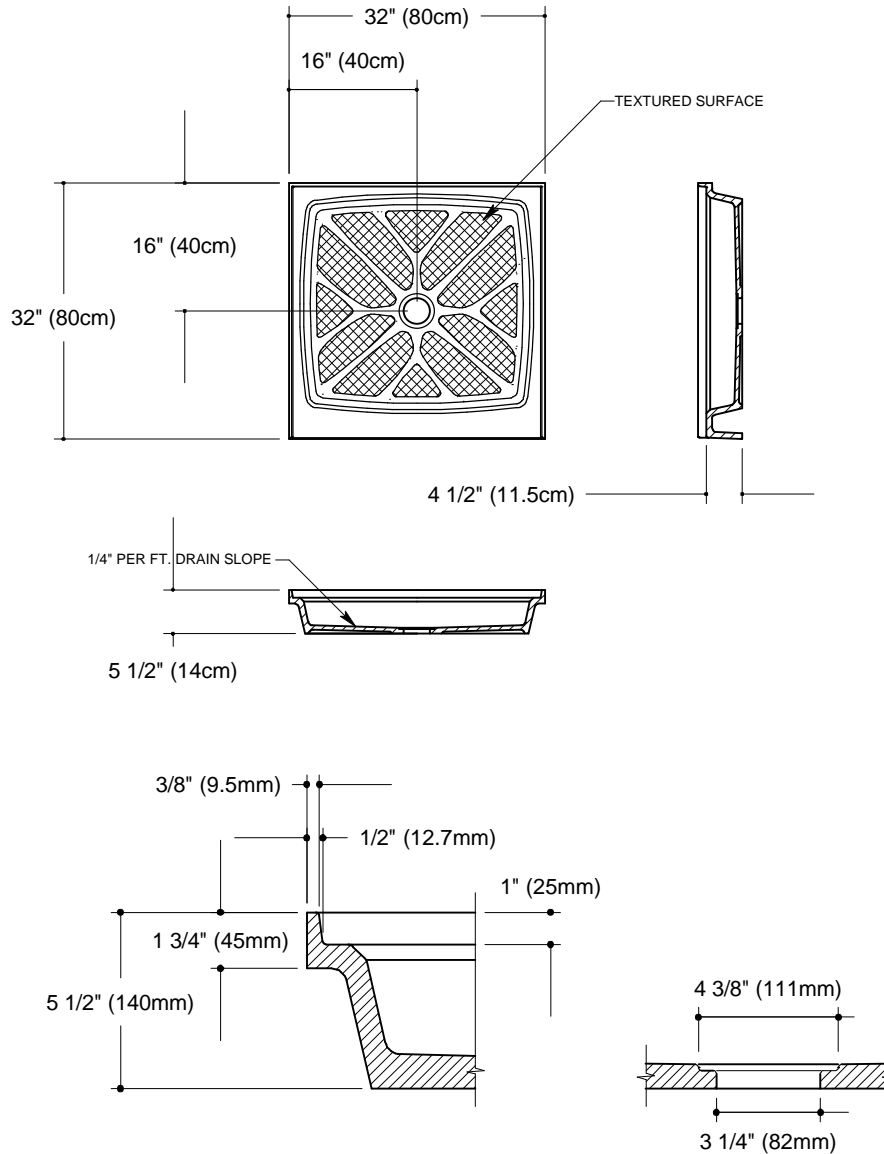
Sections showing water dam and drain details. (Lightweight option not shown)
