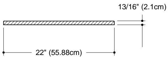
TYPICAL SECTION THROUGH THE DECK SCALE 1' = 1'0"
