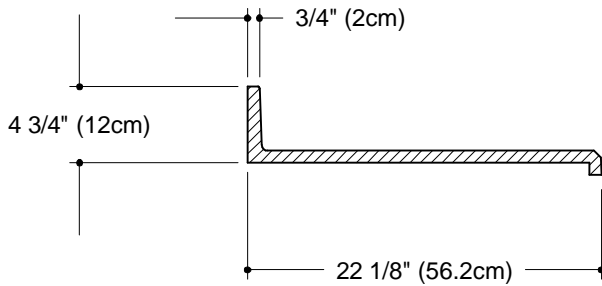
TYPICAL SECTION THROUGH THE DECK SCALE 1' = 1'0"
