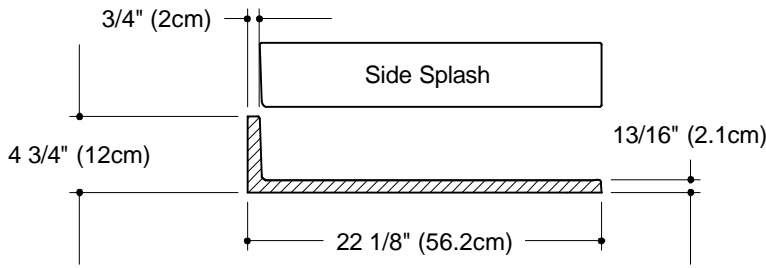
TYPICAL SECTION THROUGH THE DECK SCALE 1" = 1'0"
